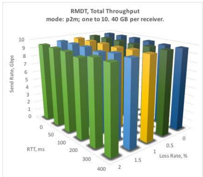
Figure 2 – Equally fast file transfer point to multiple locations using RMDT protocol
